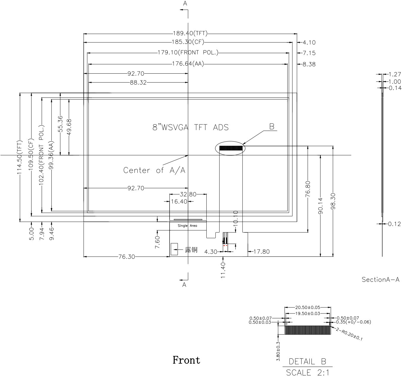
Figure 10. TFT-LCD FOG Outline Dimension (Front View)
